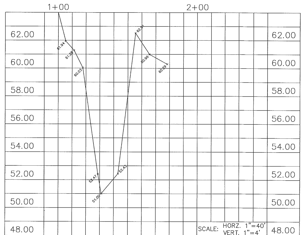
SECTION "U-U" STA. 131+70.1
