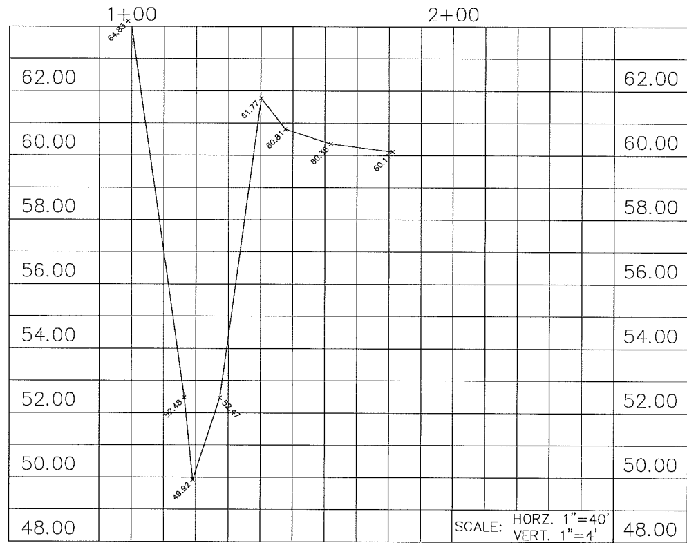
SECTION "T-T" STA. 120+67.1
