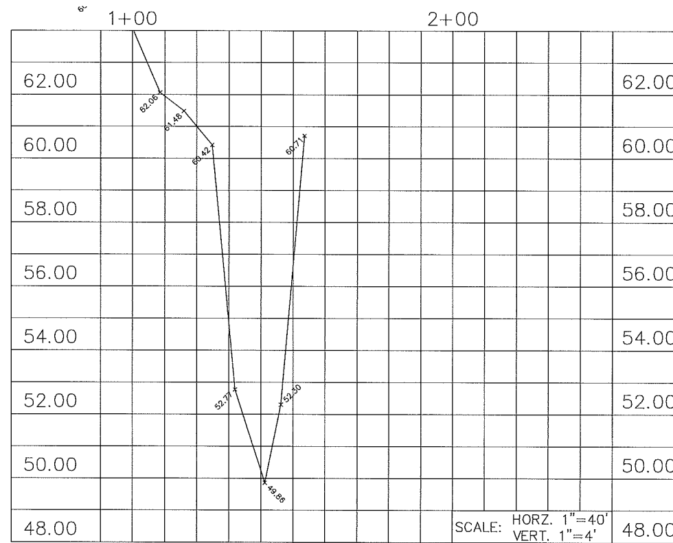
SECTION "W-W" STA. 133+11.8
