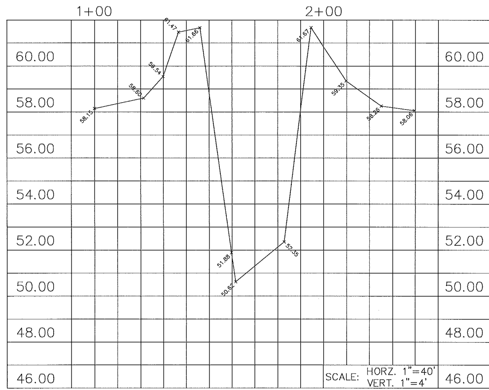
SECTION "Y-Y" STA. 6+09.2
