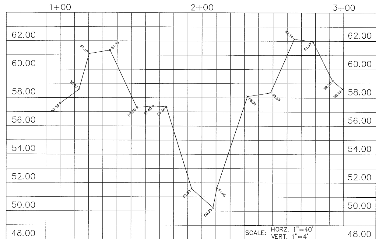
SECTION "D-D" STA. 15+94.8
