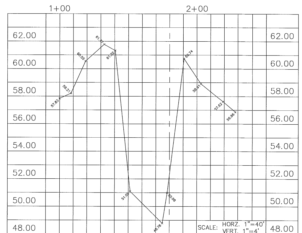
SECTION "EE-EE" STA. 13+27.8
