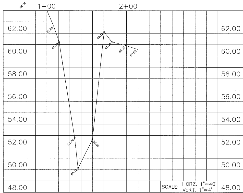
SECTION "V-V" STA. 132+33.9
