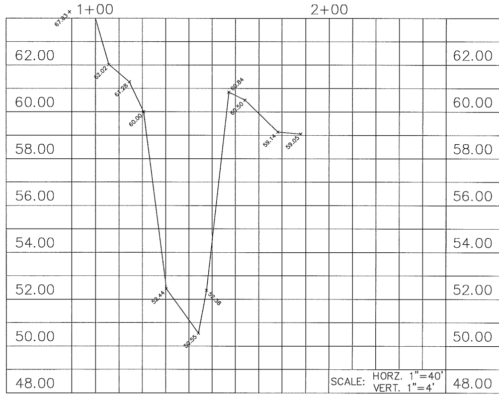
SECTION "S-S" STA. 119+88.7, LT. 79.8
